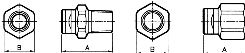
DFM ADAPTOR
