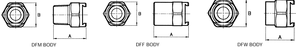
DFM BODY
